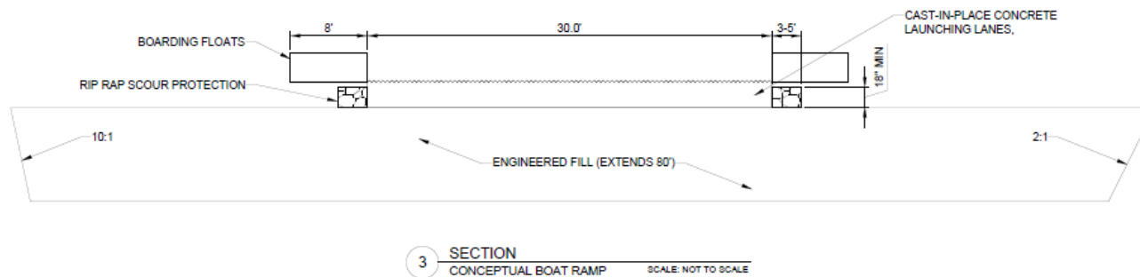
Figure 2-8. Boat Launch Facility Details
